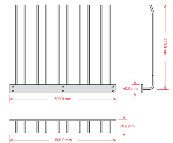
Technical Drawing
