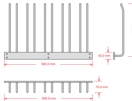
Technical Drawing
