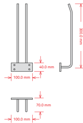
Technical Drawing
