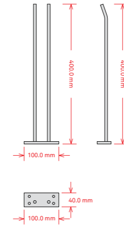
Technical Drawing
