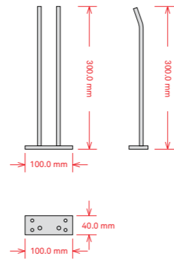
Technical Drawing
